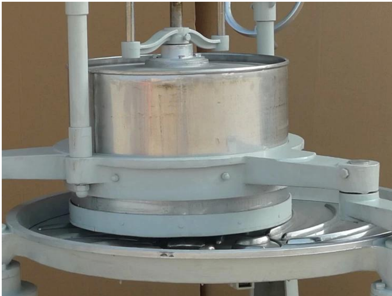
55 Type tea rolling machine, the diameter of rolling barrel is 55cm, height 40cm, can put about 35-40 kg tea in it, for green tea 1 hour can roll 35-350kg, for black tea 1 hour can roll 35-80 kg.
